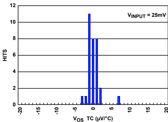
FIGURE 31. AUXILIARY V_{BUS} V_{OS} \text{ TC}
