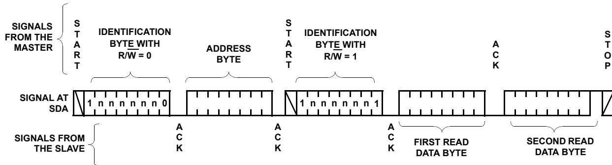
FIGURE 73. READ SEQUENCE (SLAVE ADDRESS SHOWN AS nnnn)
