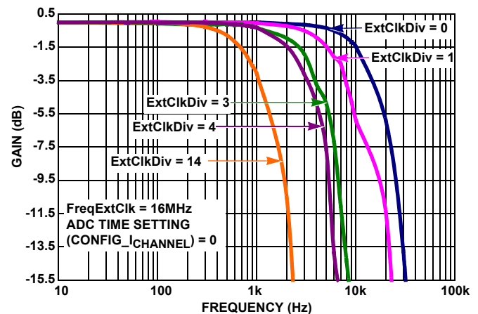
FIGURE 79. MEASUREMENT BANDWIDTH vs EXTERNAL CLK FREQUENCY
