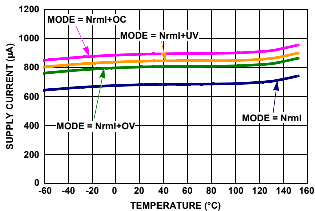
FIGURE 37. SUPPLY CURRENT vs TEMPERATURE
