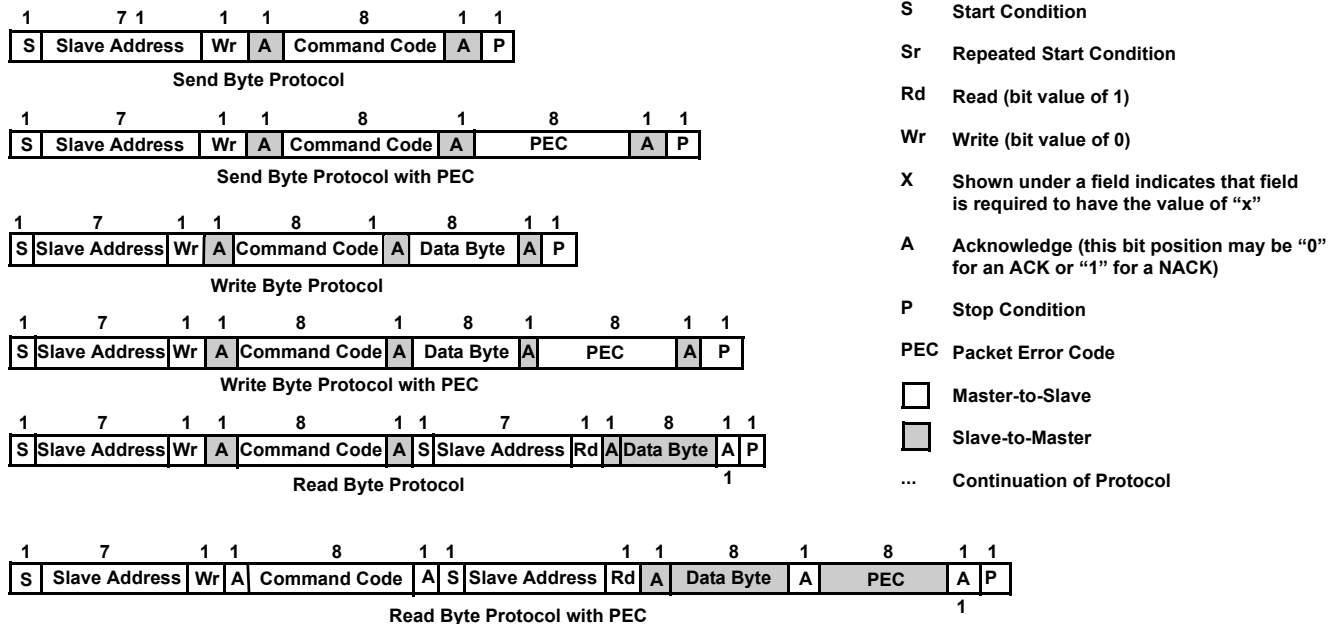
FIGURE 64. READ/WRITE SMBus PROTOCOLS WITH AND WITHOUT PEC
