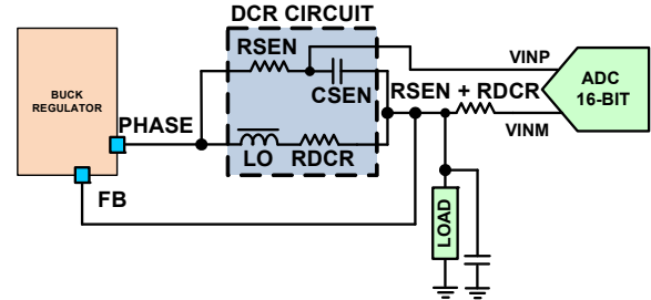
FIGURE 92. SIMPLIFIED CIRCUIT EXAMPLE OF A DCR
