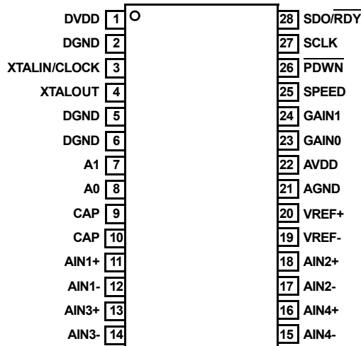
ISL26134 (28 LD TSSOP) TOP VIEW
