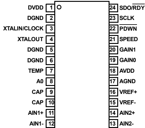
ISL26132 (24 LD TSSOP) TOP VIEW
