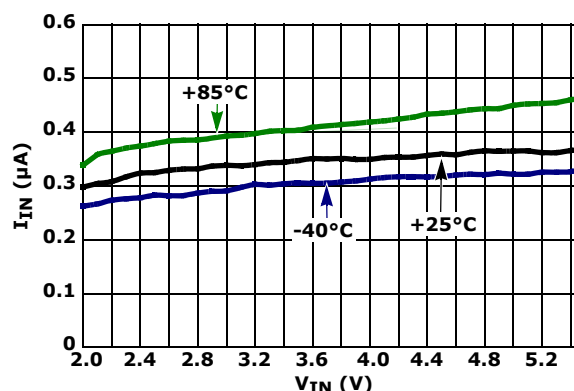
FIGURE 3. I_{IN} vs V_{IN} OVER-TEMPERATURE
