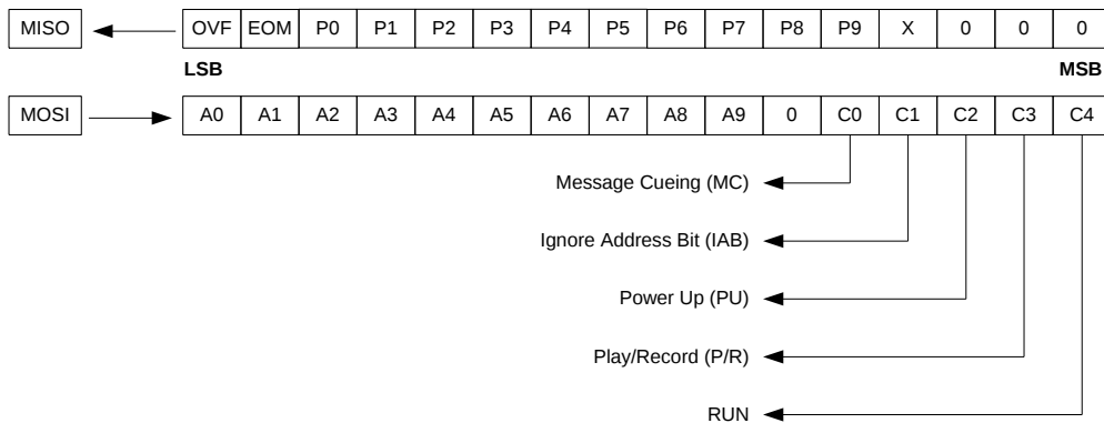
FIGURE 4: SPI PORT
