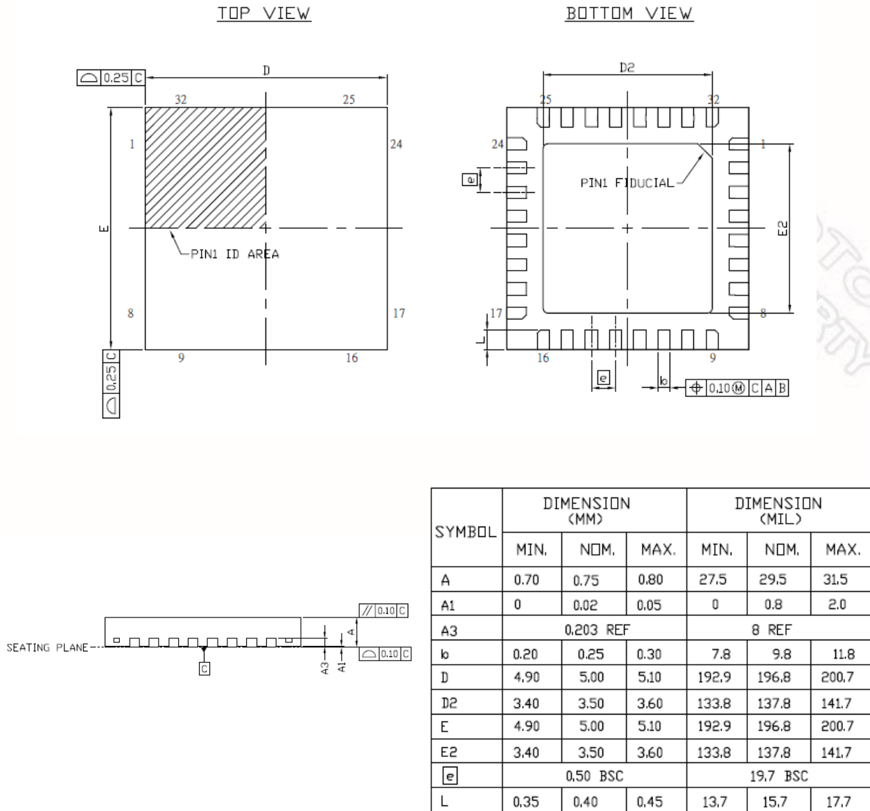
Figure 14-1 QFN 32-Lead Package
