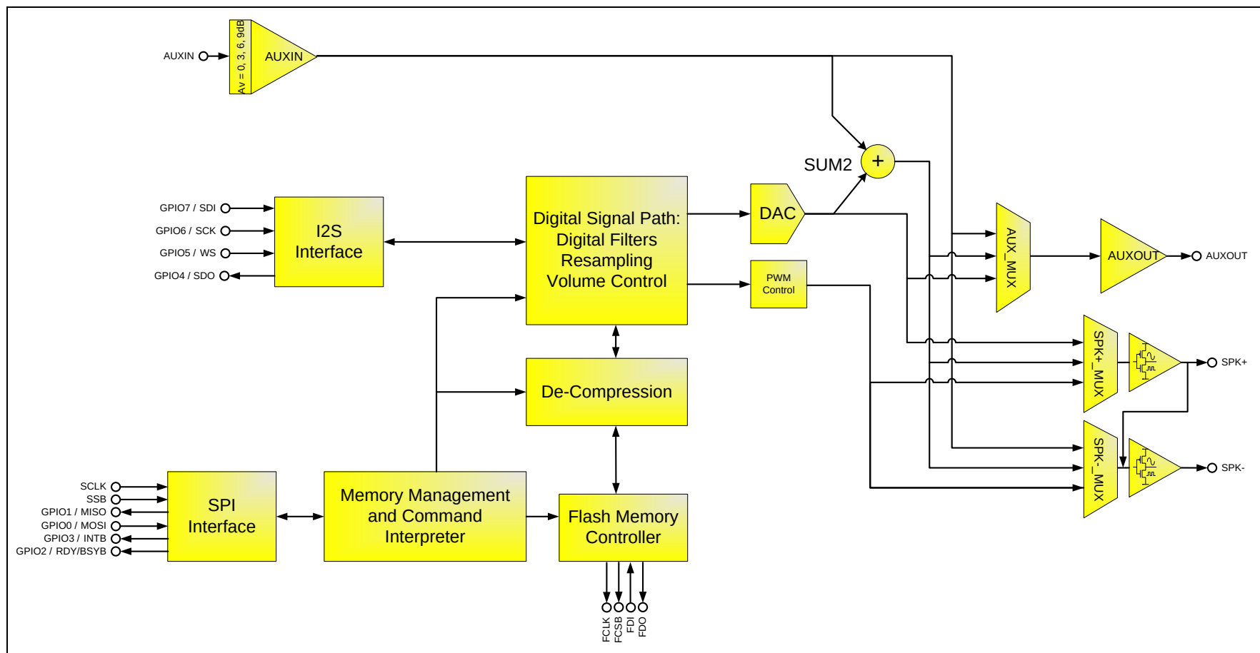
Figure 3-1 ISD15D00 Block Diagram
