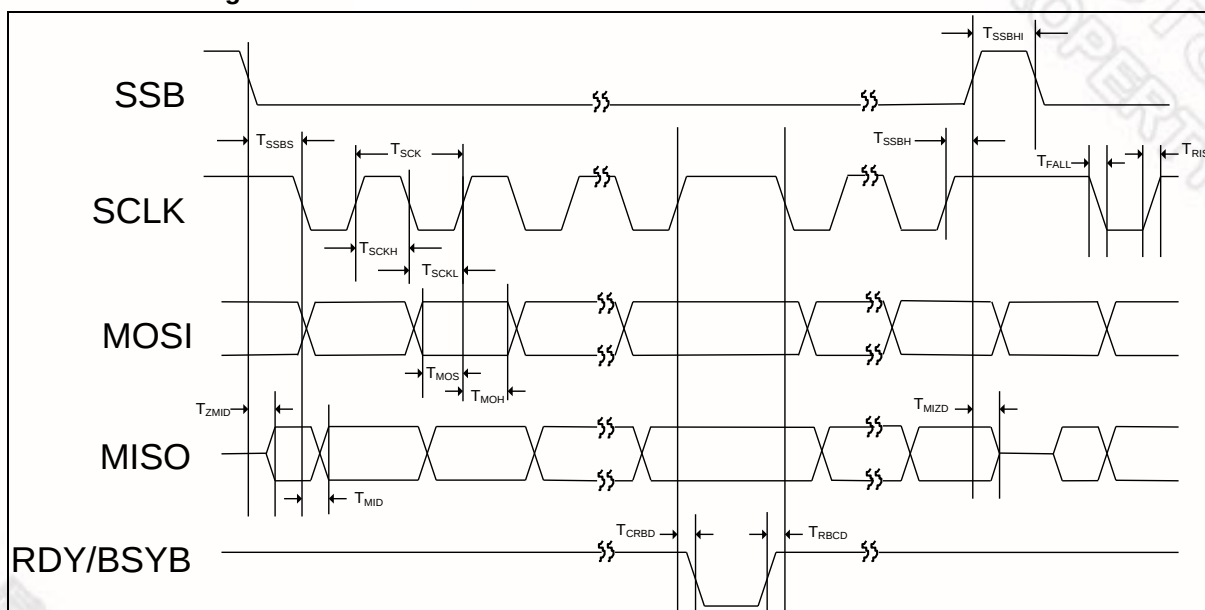
Figure 0-1 SPI Timing
