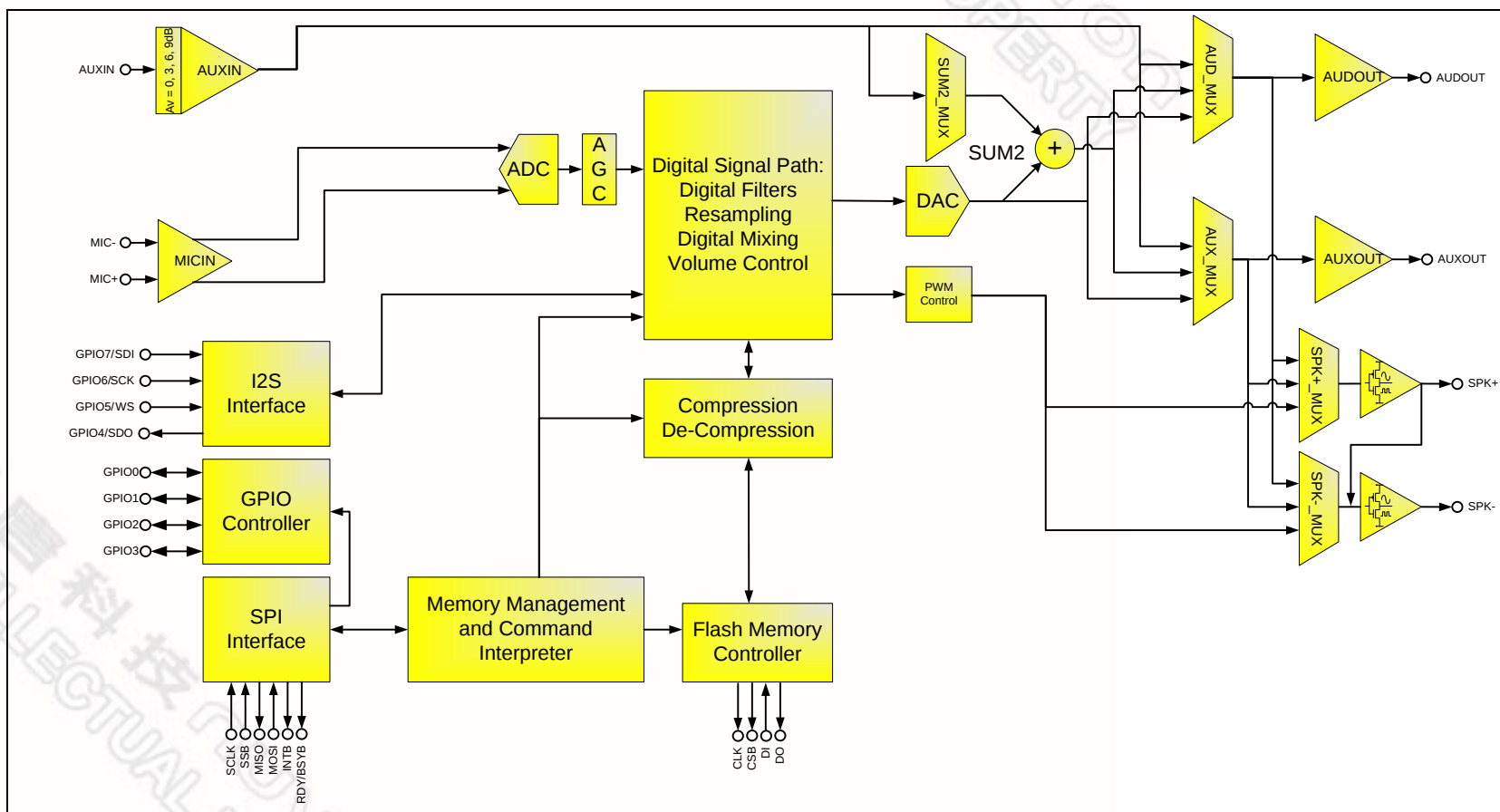
Figure 3-2 ISD15C00 Block Diagram, MICIN Selecte
