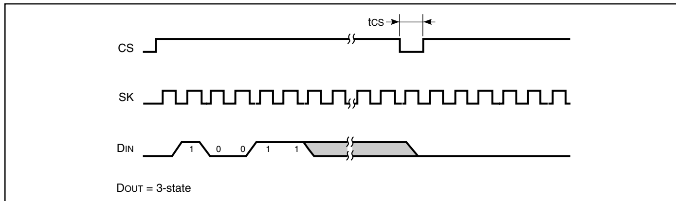
FIGURE 4. SYNCHRONOUS DATA TIMING
