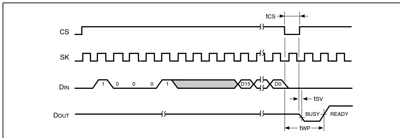
FIGURE 6. WRITE ALL (WRALL) TIMING
