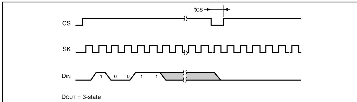
FIGURE 4. SYNCHRONOUS DATA TIMING
