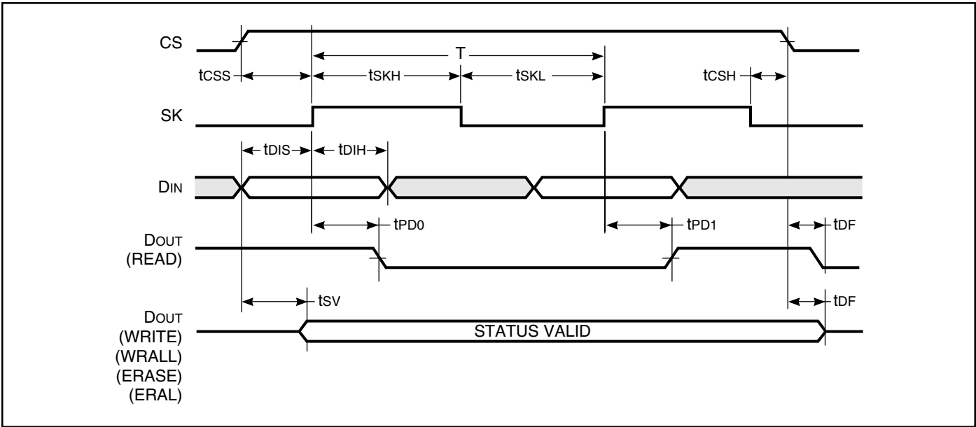
FIGURE 2. SYNCHRONOUS DATA TIMING
