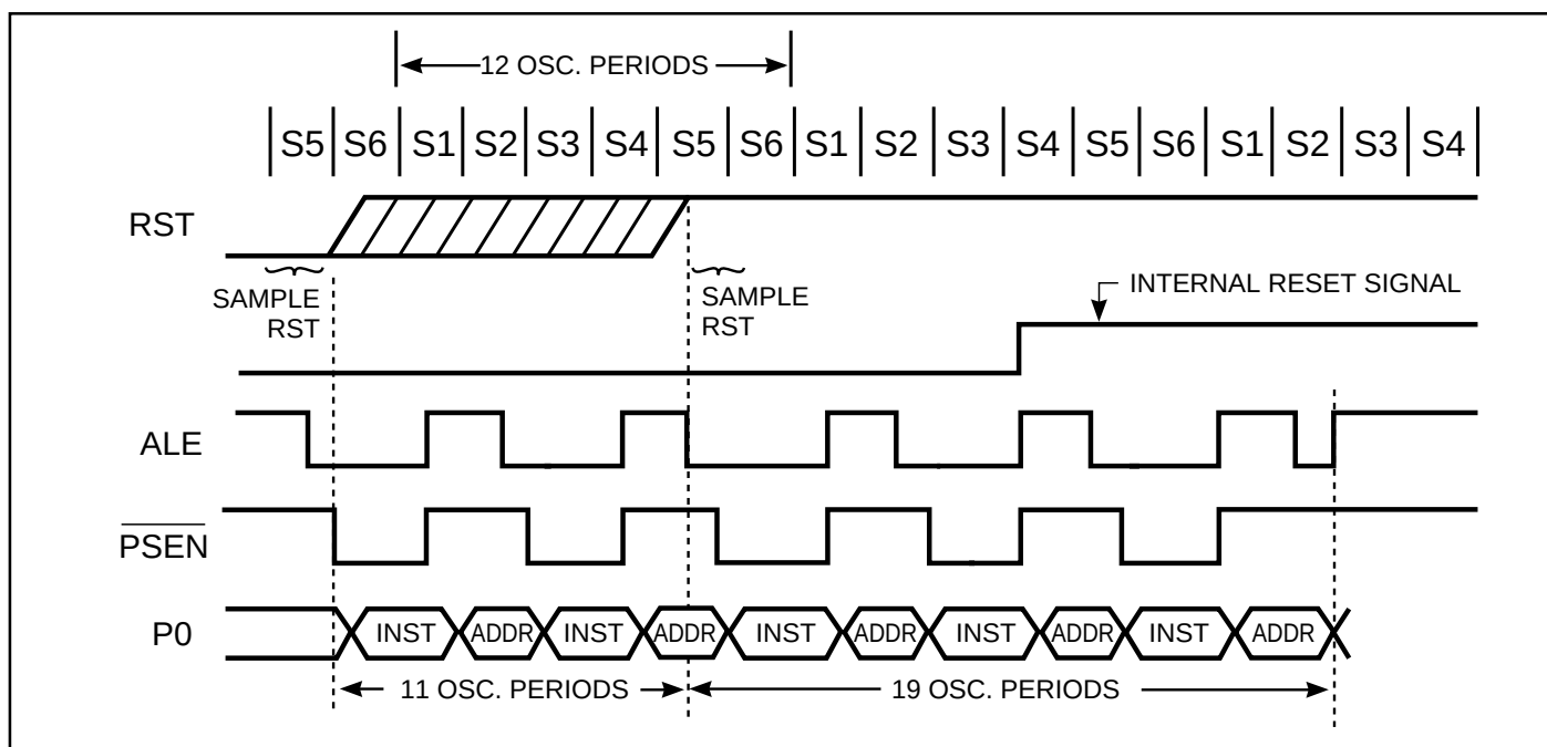
Figure 21. Reset Timing
