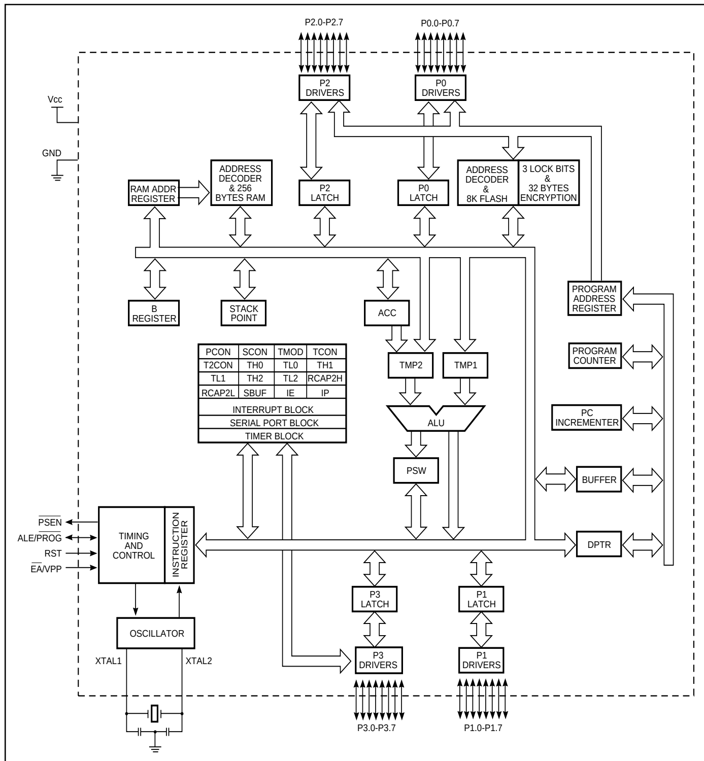
Figure 4. IS89C52 Block Diagram
