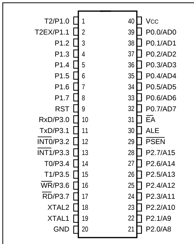
Figure 1. IS80LV52/32 Pin Configuration: 40-pin PDIP
