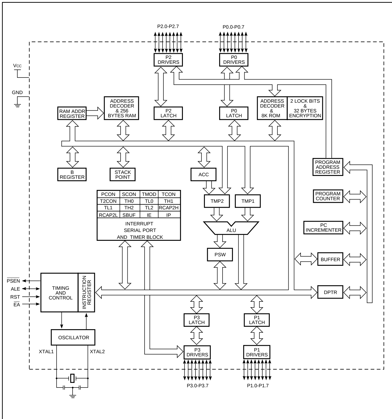
Figure 4. IS80LV52/32 Block Diagram
