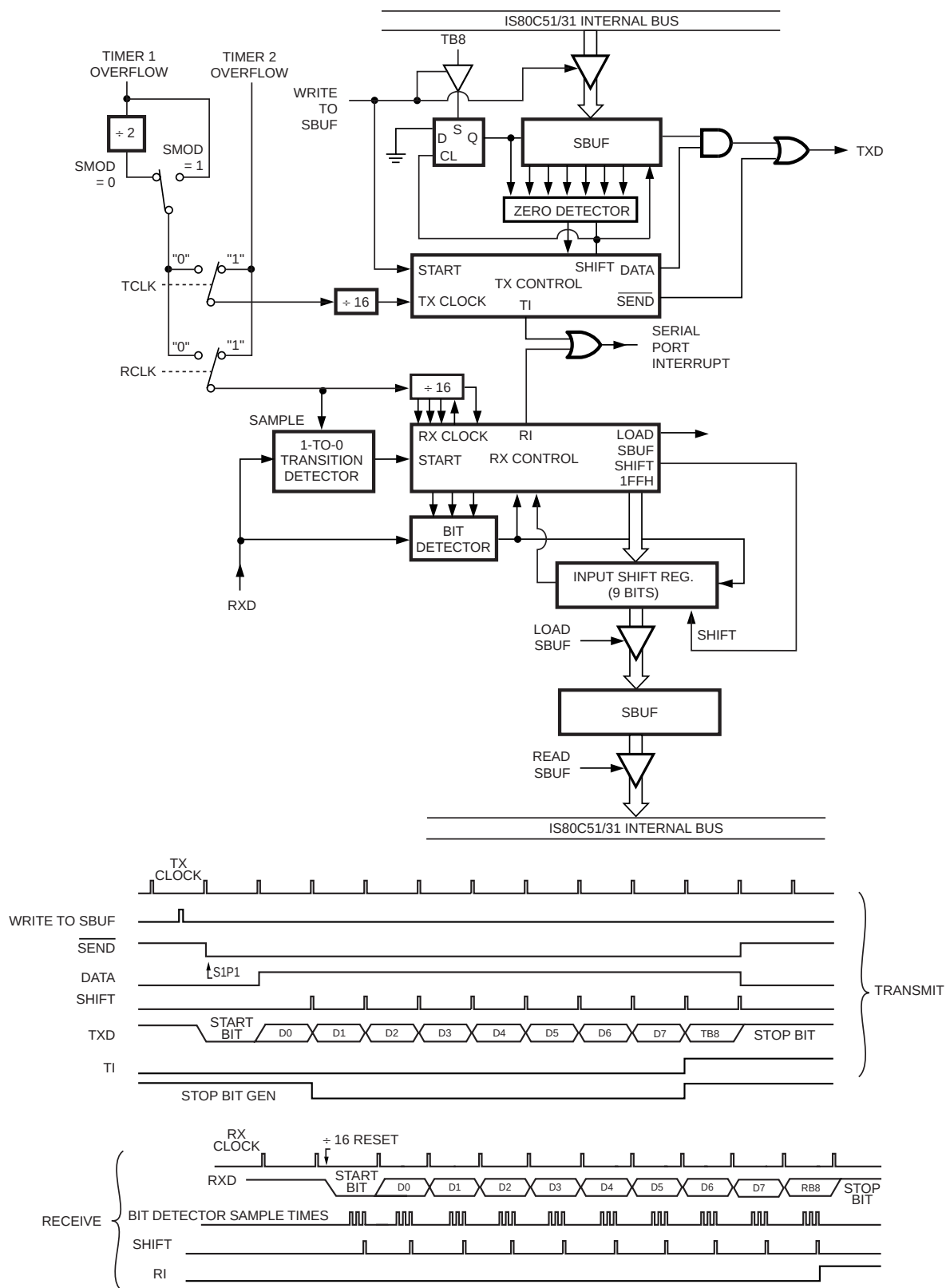
Figure 15. Serial Port Mode 3
