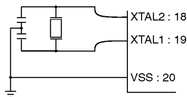
Figure 5. Crystal Oscillator.
