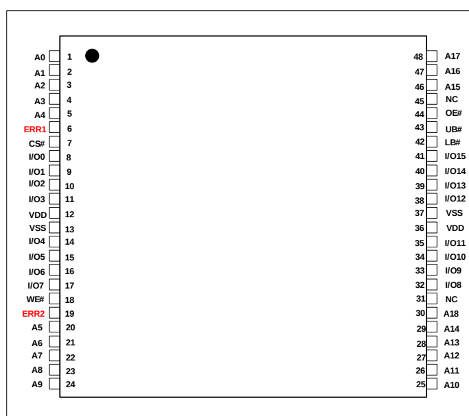
48-Pin TSOP-I, ERR1/ERR2
