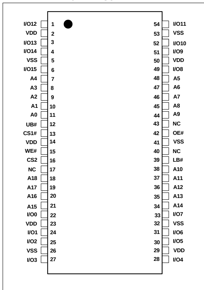
54-Pin TSOP-II
