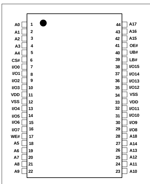
44-Pin TSOP-II
