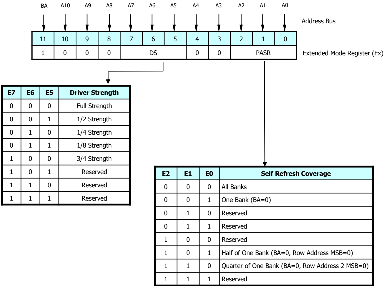
Figure5 : Extended Mode Set (EMRS) Register
