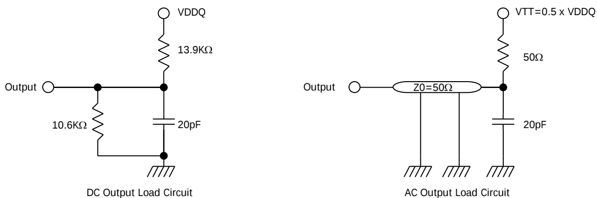
Figure8 : Output load circuit
