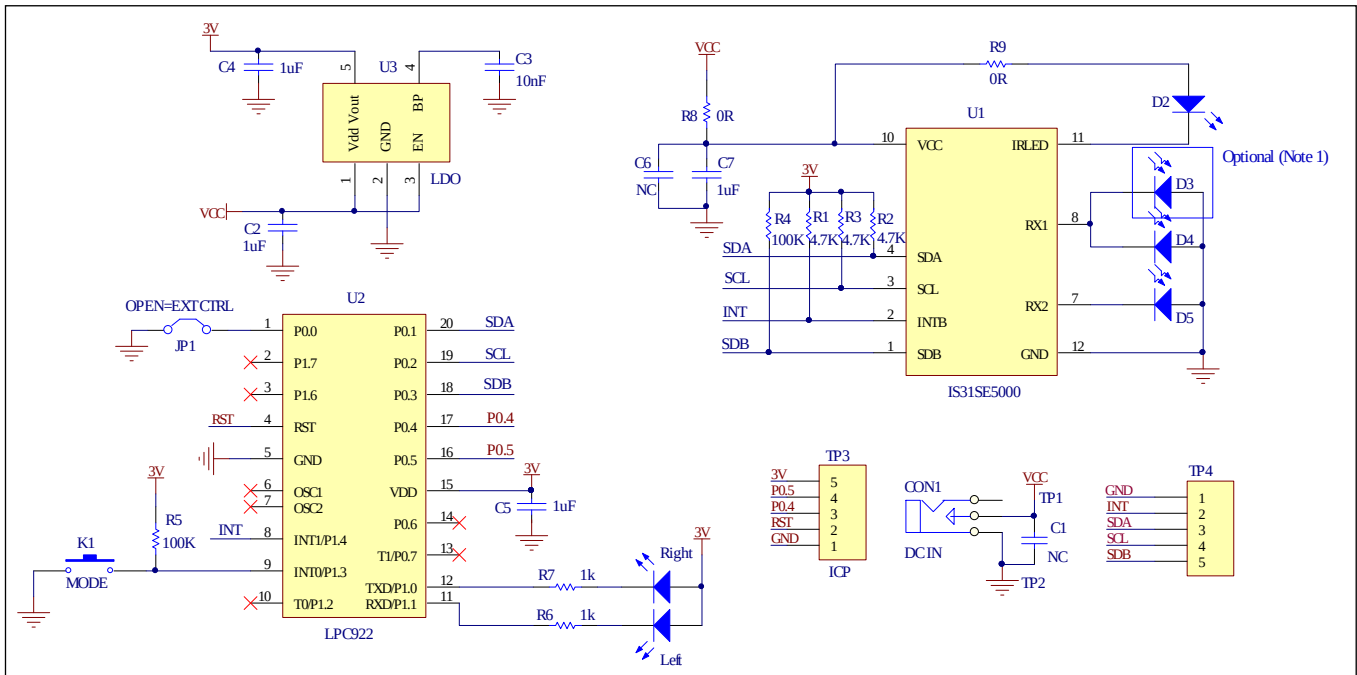
Figure 2: IS31SE5000 Application Schematic
