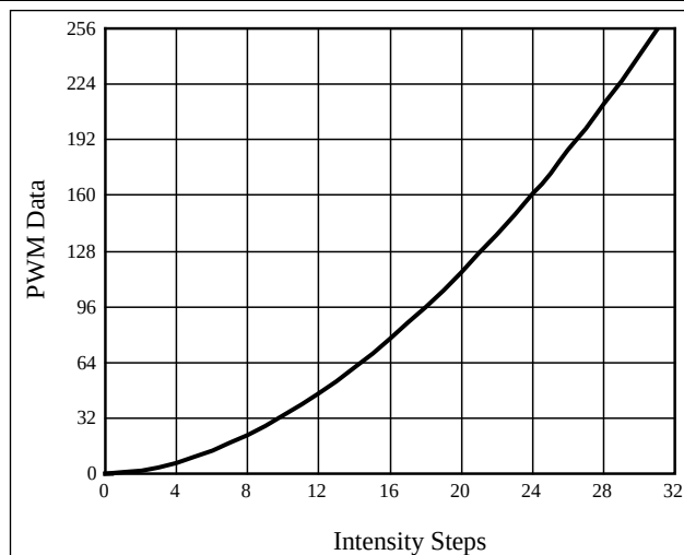
Figure 11 Gamma Correction (32 Steps)
