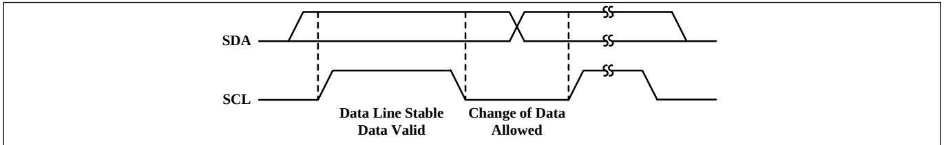
Figure 6 Bit transfer
