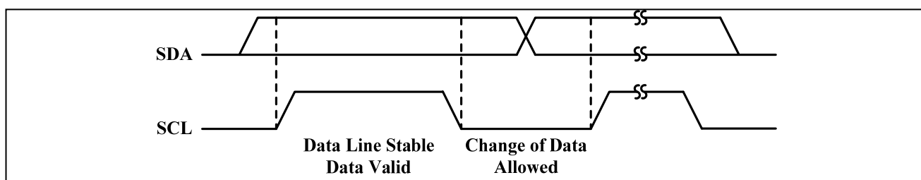
Figure 6 Bit Transfer
