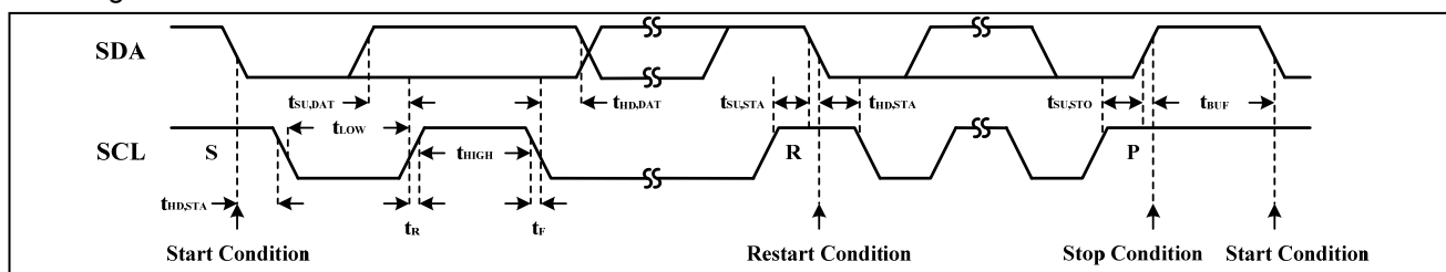
Figure 5 Interface Timing
