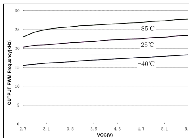
Figure 8 VCC vs. OUTPUT PWM Frequency
