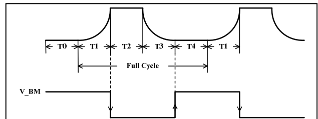
Figure 8 V BM Signal
