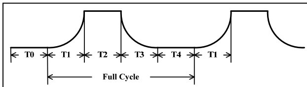
Figure 7 Breathing Timing
