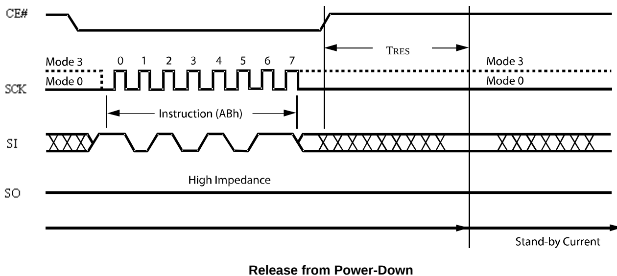
Figure 5. Read Device ID (Top Diagram) and Release from Power-Down (Bottom Diagram)
