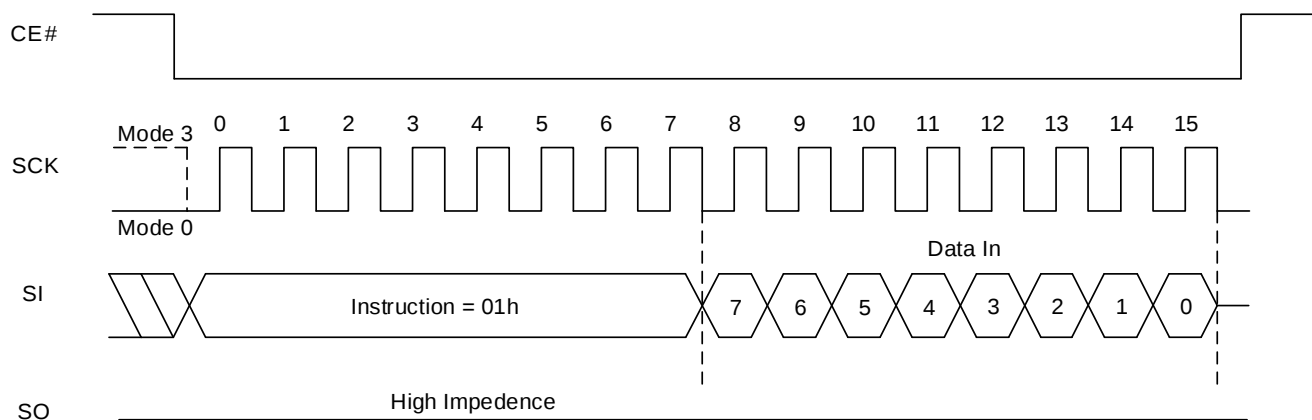
Figure 8.47 Write Status Register Sequence In SPI Mode
