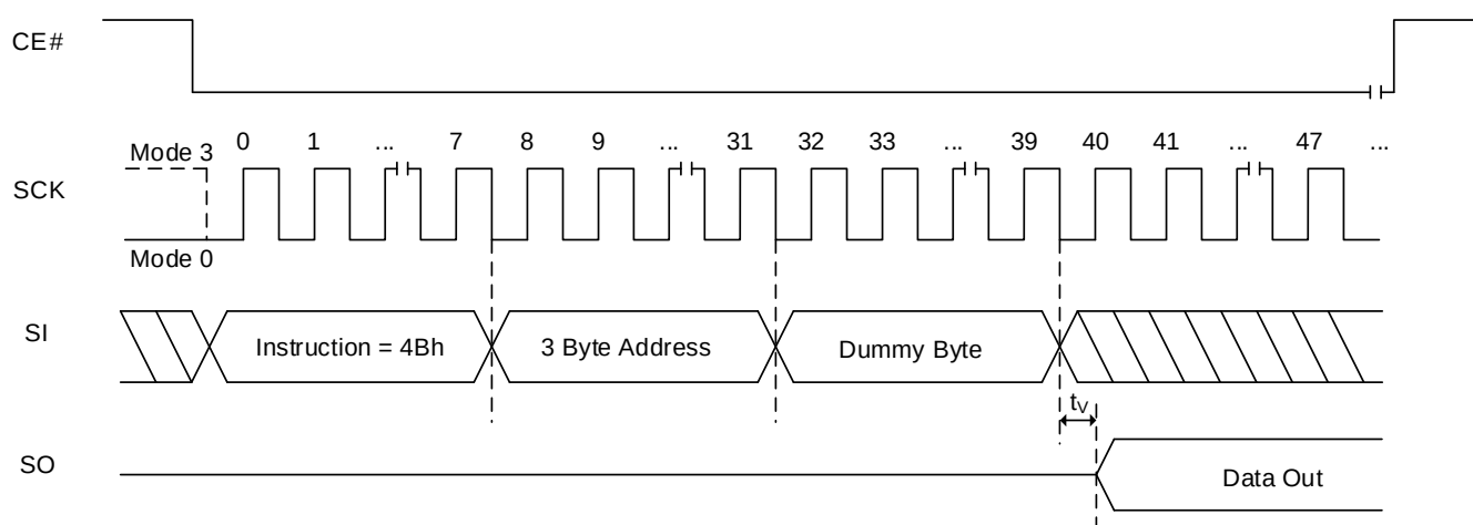
Figure 8.48 RDUID Sequence
