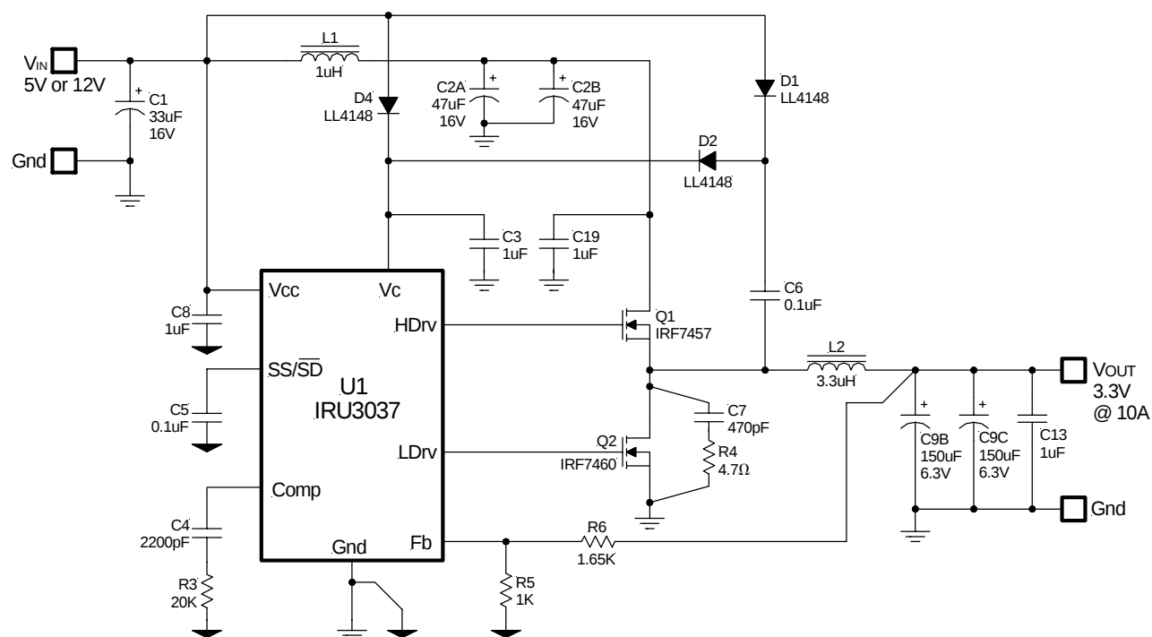
Figure 20 - Demo-board application of IRU3037.
