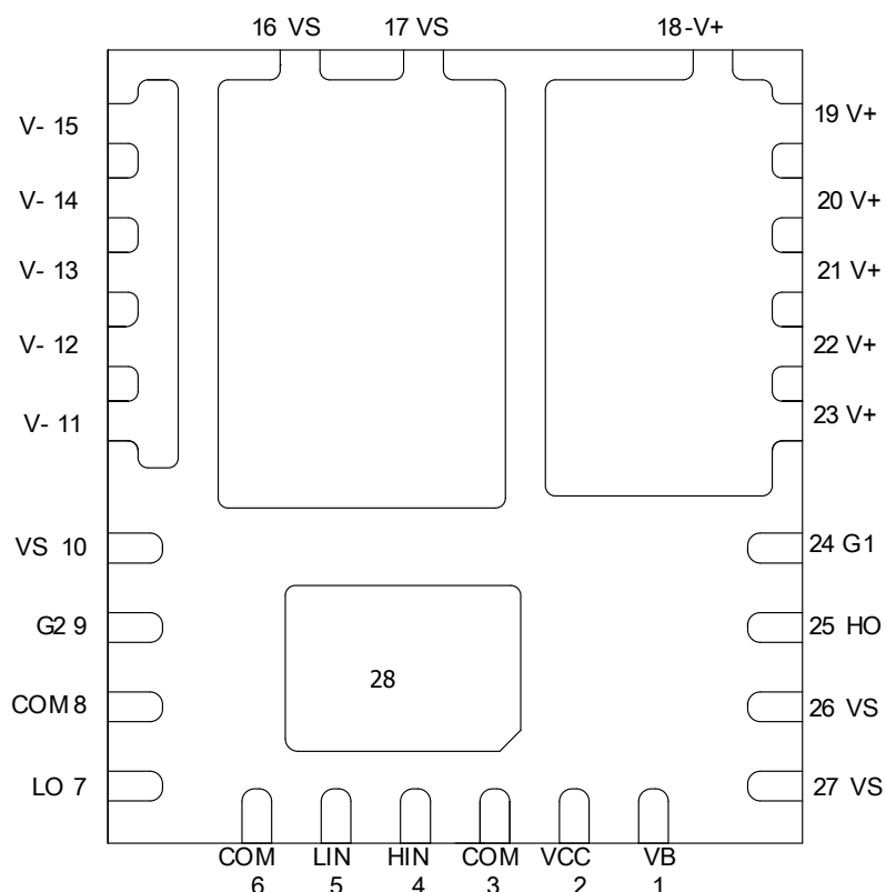
BOTTOM OF PACKAGE VIEW
