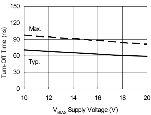
Figure 7B. Turn-Off Time vs. Supply Voltage
