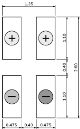
Pyroelectric Element
