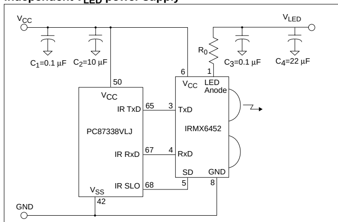
Figure 8. Super I/O (PC87338VLJ) to IRMS6452/IRMT6452 with independent V_{LED} power supply
