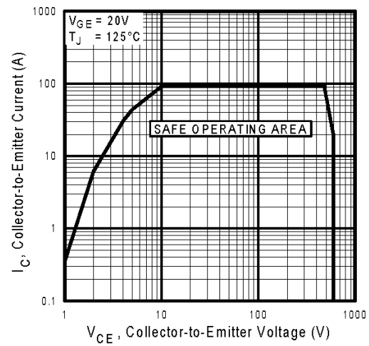
Fig. 12 - Turn-Off SOA
