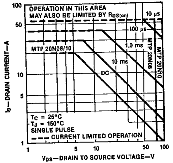
Figure 11 Forward Biased Safe Operating Area for MTP20N08/20N10
