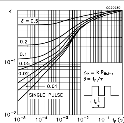
Figure 2. Thermal impedance for TO-220/ DPAK/ D 2 PAK
