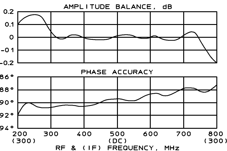
Performance over Video Bandwidth (LO at 500 MHz)
