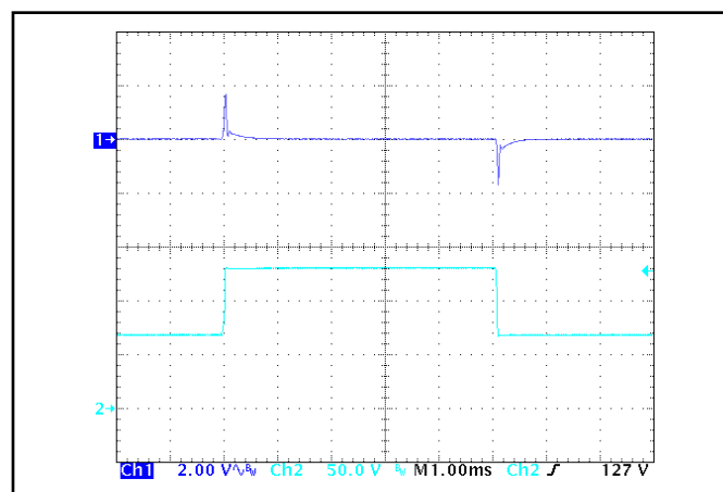
Figure 6: Output voltage response to step-change in input voltage (500 V/ms). Load cap: 100 μF, electrolytic output capacitance. Ch 1: V out (2 V/div), Ch 2: V in (50 V/div).
