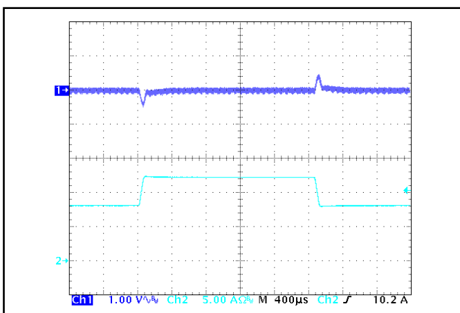
Figure 5: Output voltage response to step-change in load current (50%-75%-50% of Iout(max); dI/dt = 0.1 A/μs). Load cap: 15 μF Tantalum + 1 μF Ceramic capacitor. Ch 1: Vout (1 V/div), Ch 2: Iout (5 A/div).
