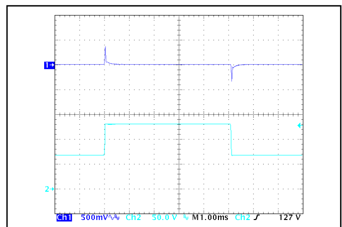
Figure 6: Output voltage response to step-change in input voltage (500 V/ms). Load cap: 100 μF, electrolytic output capacitance. Ch 1: V out (500 mV/div), Ch 2: V in (50 V/div).
