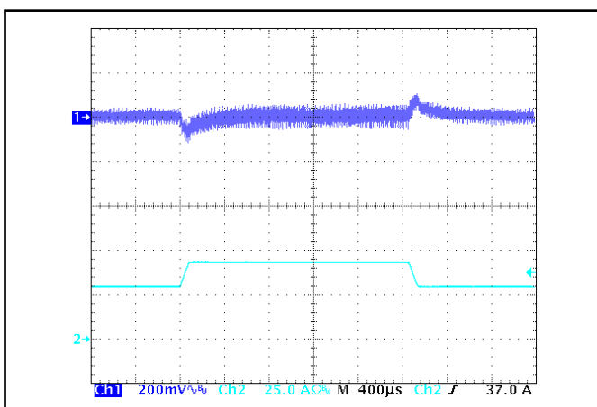
Figure 5: Output voltage response to step-change in load current (50%-75%-50% of I out (max); dI/dt = 0.1 A/μs). Load cap: 15 μF Tantalum + 1 μF Ceramic capacitor. Ch 1: V out (200 mV/div), Ch 2: I out (25 A/div).
