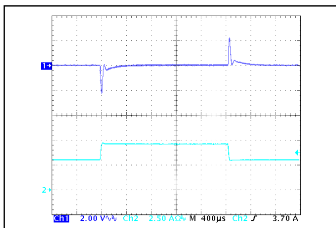
Figure 5: Output voltage response to step-change in load current (50%-75%-50% of I out (max); dI/dt = 0.1 A/μs). Load cap: 1 μF ceramic capacitor. Ch 1: V out (2 V/div), Ch 2: I out (2.5 A/div).
