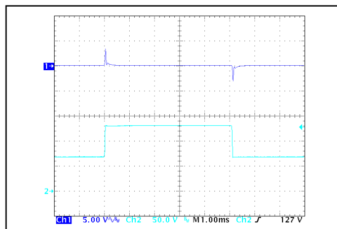
Figure 6: Output voltage response to step-change in input voltage (500 V/ms). Load cap: 100 μF electrolytic output capacitance. Ch 1: V out (5 V/div), Ch 2: V in (50 V/div).
