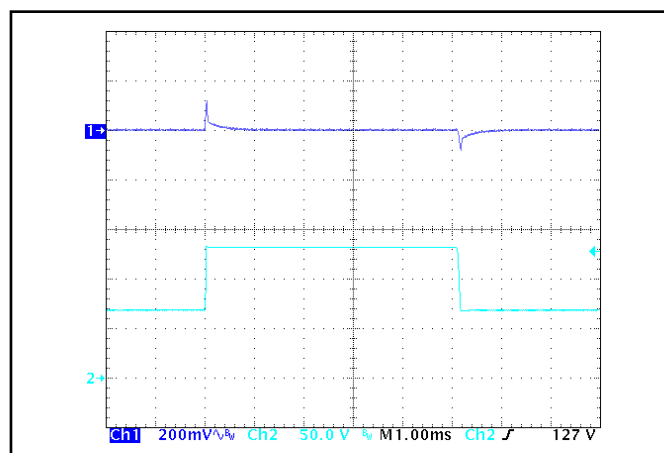
Figure 6: Output voltage response to step-change in input voltage (500 V/ms). Load cap: 100 μF, electrolytic output capacitance. Ch 1: V out (200 mV/div), Ch 2: V in (50 V/div).
