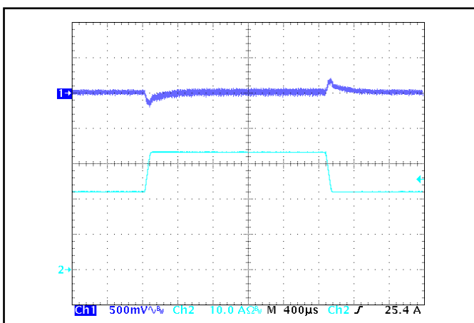
Figure 5: Output voltage response to step-change in load current (50%-75%-50% of I out (max); dI/dt = 0.1 A/μs). Load cap: 15 μF Tantalum + 1 μF Ceramic capacitor. Ch 1: V out (500 mV/div), Ch 2: I out (10 A/div).
