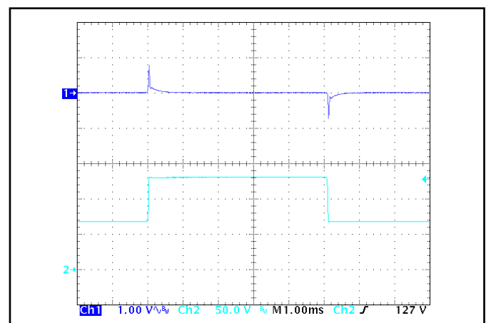
Figure 6: Output voltage response to step-change in input voltage (500 V/ms). Load cap: 100 μF, electrolytic output capacitance. Ch 1: V out (1 V/div), Ch 2: V in (50 V/div).
