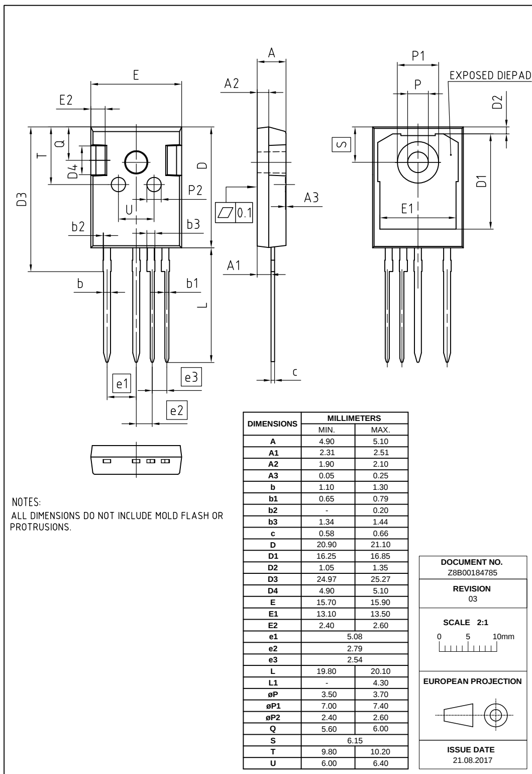
Figure 1 Outline PG-TO 247-4-3, dimensions in mm
