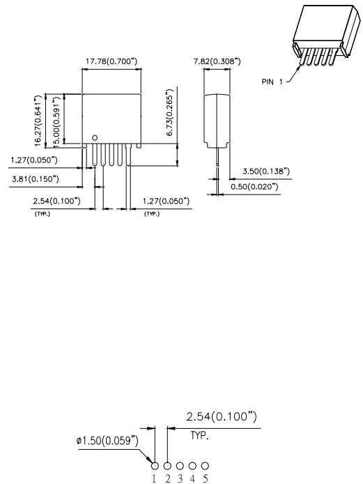
RECOMMEND PWB HOLE LAYOUT
