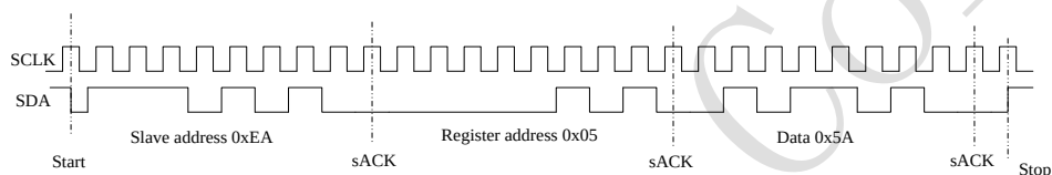
I2C WRITE
