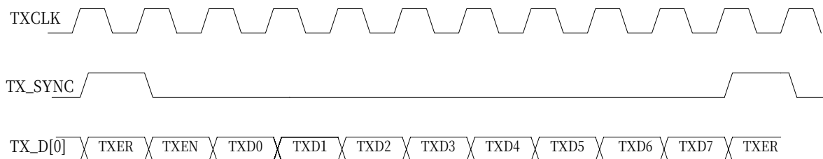
Transmit SS-SMII
