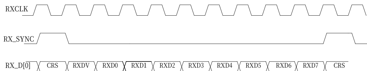
Receive SS-SMII
