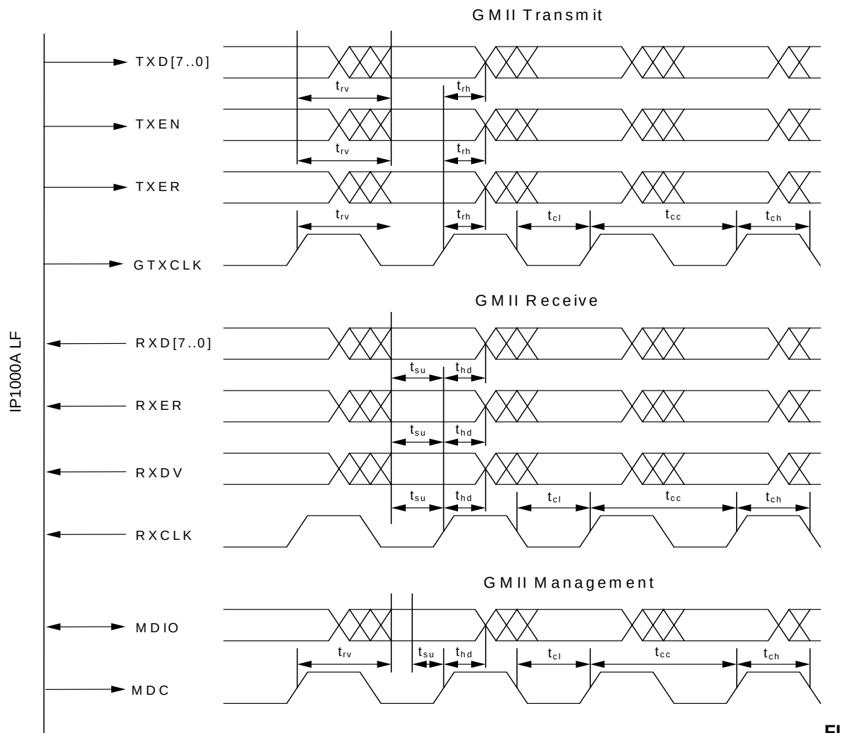
FIGURE 7-4: GMII Switching Characteristics
