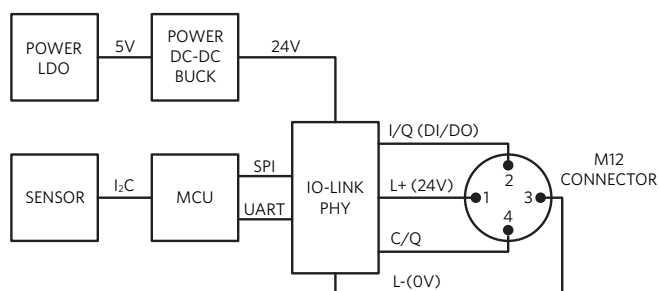
Figure 17. Building Blocks of an IO-Link Sensor
