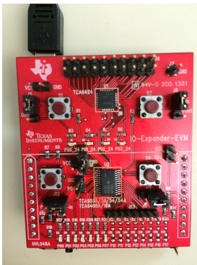
Figure 1. IO Expander EVM
