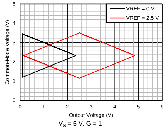
Figure 48. Input Common-Mode Voltage vs Output Voltage
