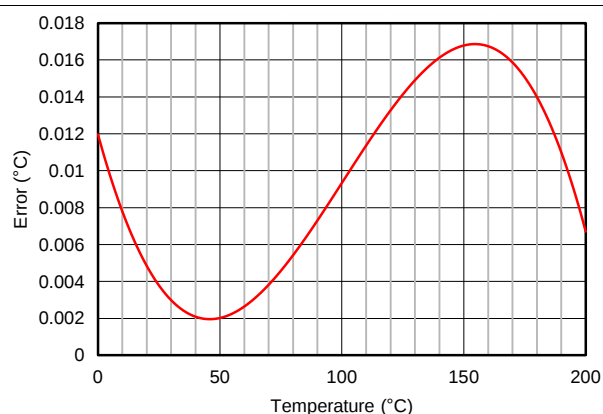
Figure 73. Temperature Error Over Full Temperature Range
