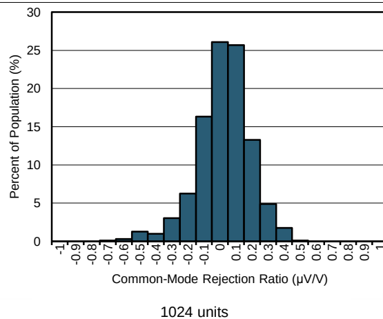
Figure 8. Typical Distribution of CMRR (G = 100)
