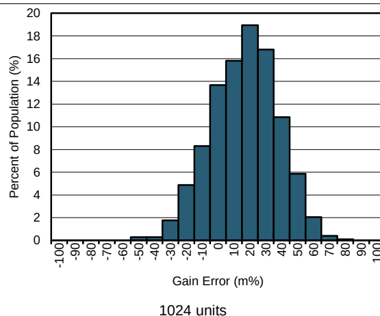
Figure 10. Gain Error (G = 10)
