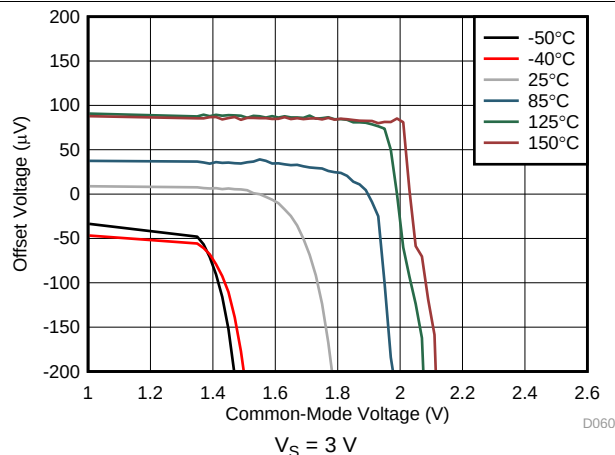
Figure 47. Offset Voltage vs Positive Common-Mode Voltage
