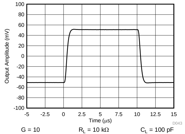
Figure 44. Small-Signal Response
