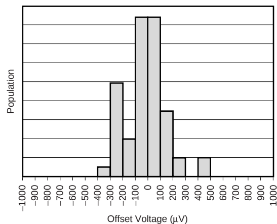
OFFSET VOLTAGE PRODUCTION DISTRIBUTION G = 10
