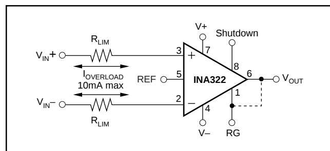
FIGURE 7. Input Protection.
