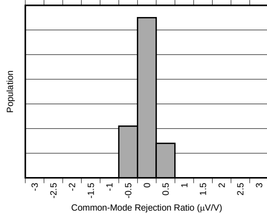
Figure 7. CMRR Distribution (INA30xA3-Q1)
