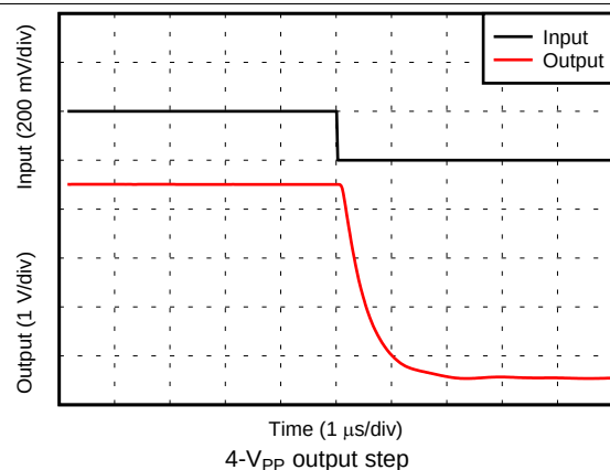
Figure 25. Voltage Output Falling Step Response
