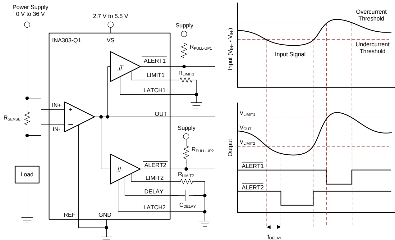
Figure 43. Out-of-Range Alert Responses for the INA303-Q1
