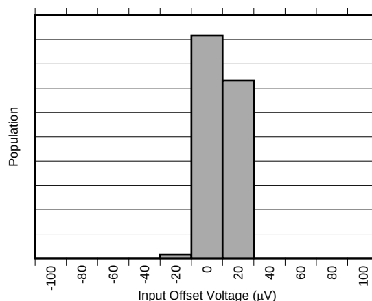
Figure 2. Input Offset Voltage Distribution (INA30xA2-Q1)
