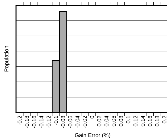
Figure 10. Gain Error Distribution (INA30xA1-Q1)
