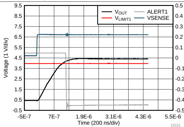
Figure 31. Comparator 1 Total Propagation Delay (INA30x-Q1)
