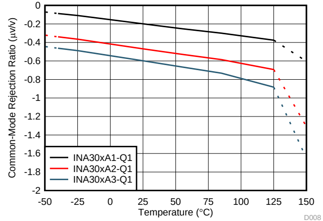
Figure 8. CMRR vs Temperature
