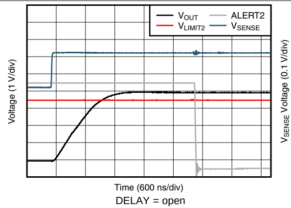
Figure 32. Comparator 2 Total Propagation Delay (INA303-Q1)
