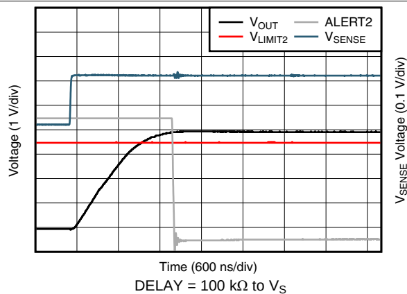
Figure 33. Comparator 2 Total Propagation Delay (INA303-Q1)
