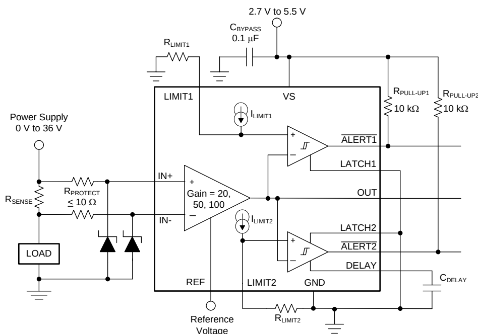
Figure 51. Transient Protection
